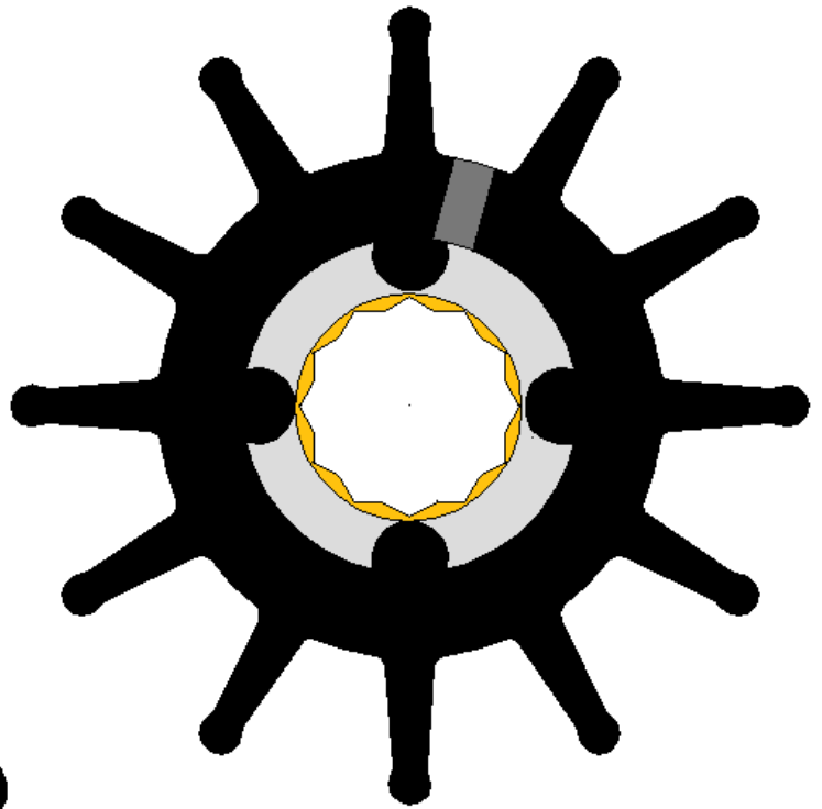
Cod. 5288: De 95 - H 95.0 - Di 25, Neoprene, Ins. 4
