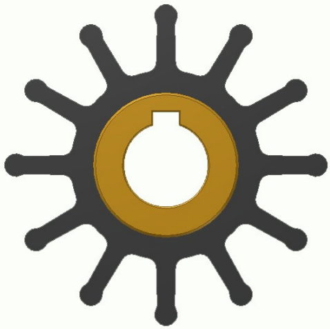
Cod. 4988: De 61.9 - H 22.2 - Di 16, Neoprene, Ins. 3
