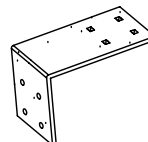
PSLM Platform Swing Ladder Mount for Adapting Swing Mount to Platform Application
